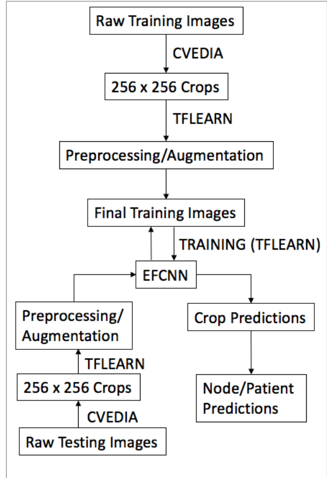
Fig. 1. Outline of full algorithm
