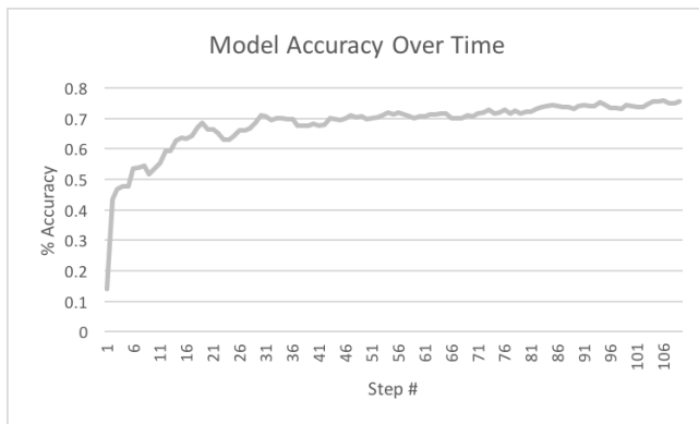
Fig. 3. Model Accuracy
