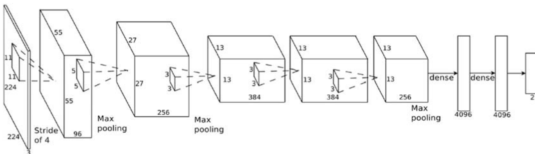
Figure 2 Architecture of the AlexNet CNN
